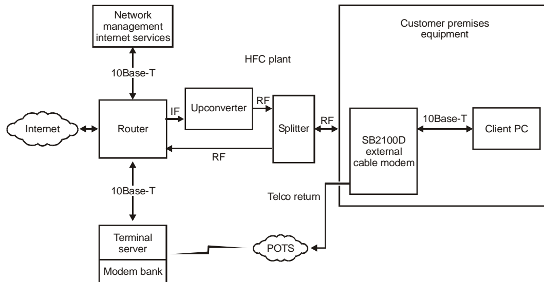
Figure 2-1 SB2100D data path
